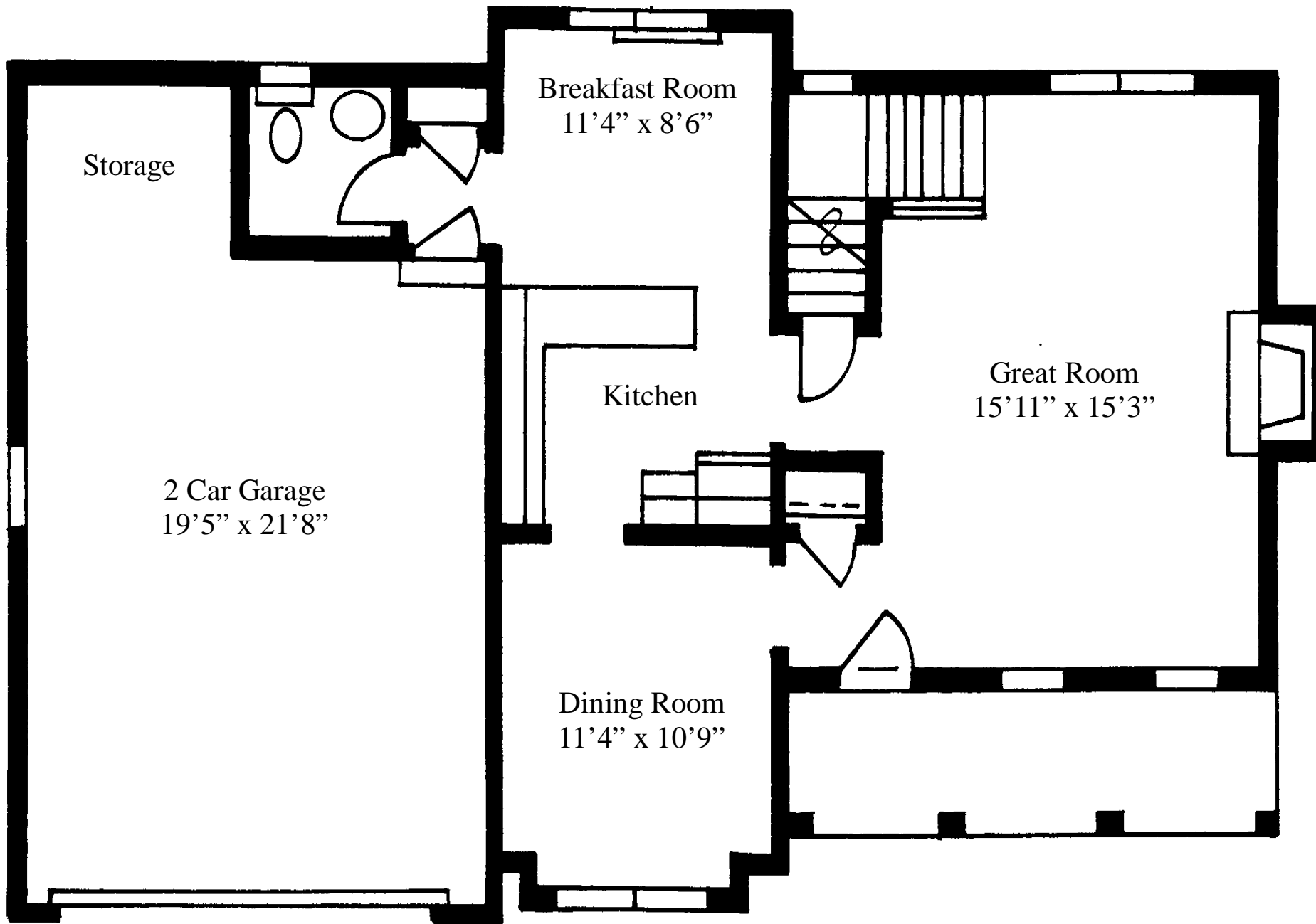
FIRST FLOOR PLAN 1630
